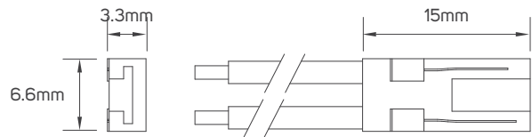
614033 - Connector
