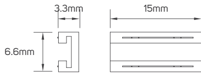
614032 - Connector
