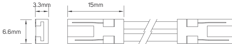
614034 - Connector
