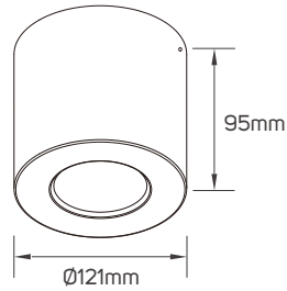
613126 - 613127 - Surface Mounted Kit
