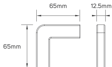
613557 - L Connector
